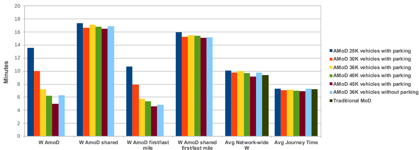
Figure 10: Waiting time (W) across automated on-demand modes for the different scenarios (in minutes). Avg Network-Wide W is the average W over buses, trains and MoD. Journey Time captures average travel time across all modes.
