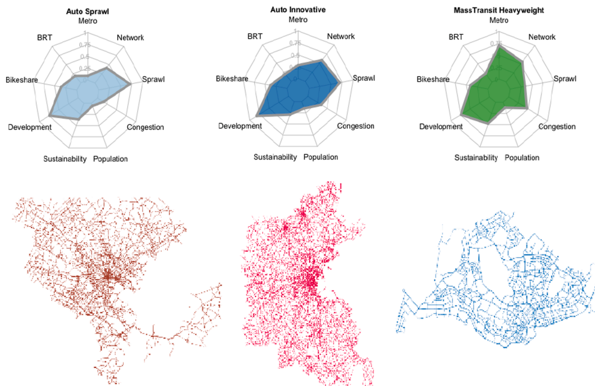
Fig. 1. The three typologies used for simulation and equity analysis: Auto Sprawl , Auto Innovative and MassTransit Heavyweight . Factor profiles (spider plots) are shown in the top row, while the respective archetype city networks used in the simulation are shown below. The “Network” label represents “Network Density.”
