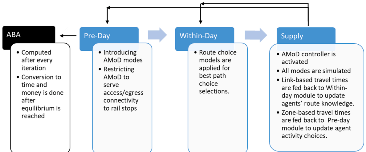
Fig. 2. SimMobility-MT components and ABA computation process.
